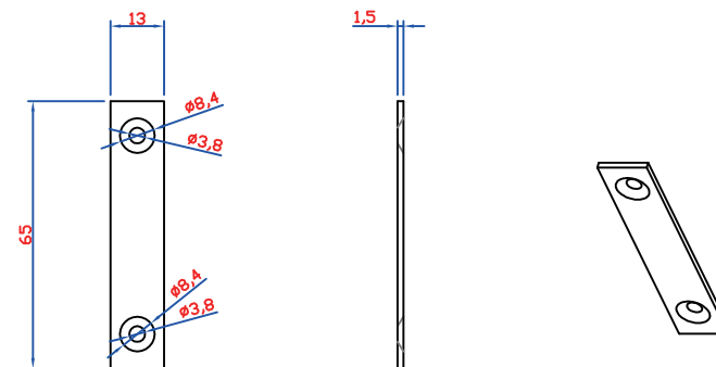
F3 Iron Sheet 1PC In Accessories Bag 门锁方铁片 * 1件 用途:五金包
